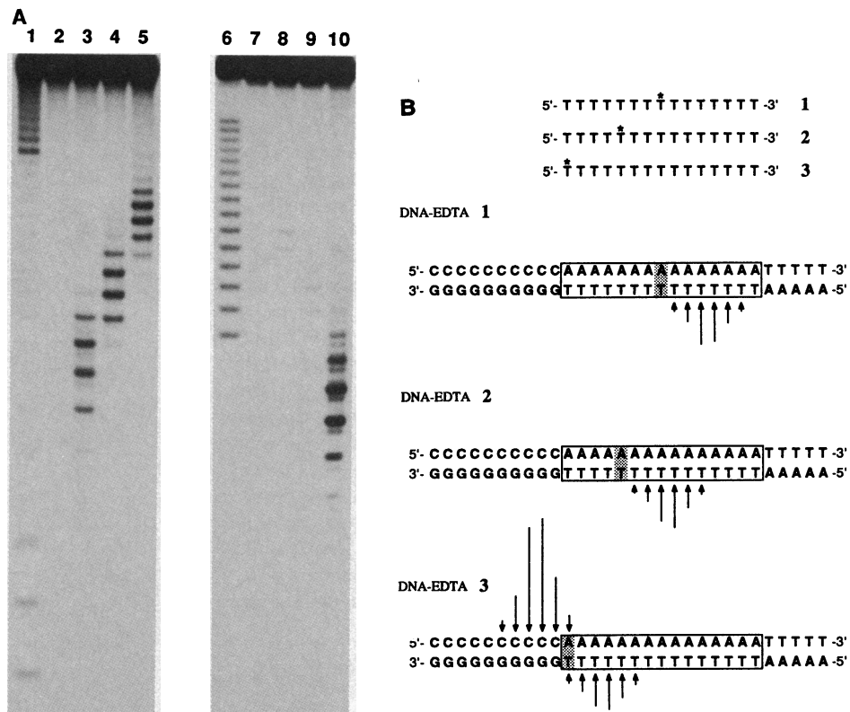
Fig. 2. Oligonucleotide-directed cleavage of double helical DNA by a triple helix-forming DNA-EDTA·Fe probe. One thymidine has been replaced by thymidine with the iron chelator EDTA covalently attached at C-5. Reduction of dioxygen generates localized hydroxyl radical at this position (26).
